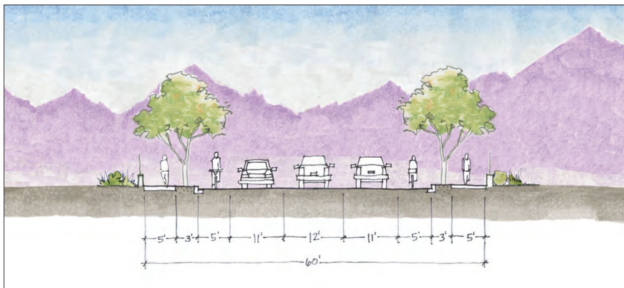
Figure 4.29: Avenue 50 west of Harrison Street – Proposed 60' Segment
