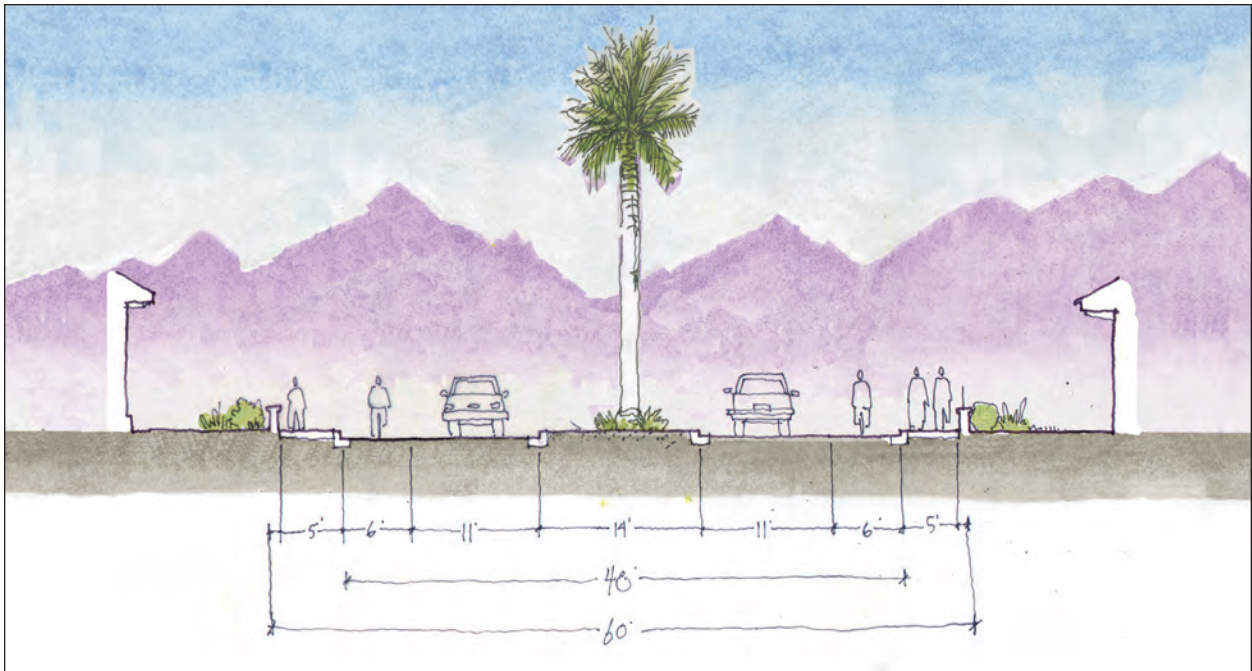
Figure 4.31: Avenue 52 — Proposed
